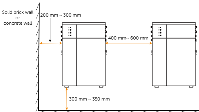
Elevation view of wall mounting
