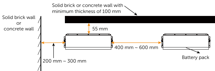
Plan view of floor mounting/wall mounting
