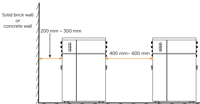
Elevation view of floor mounting
